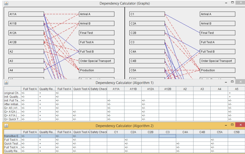
Fig. 8. Proof-of-concept prototype (Screenshots)
