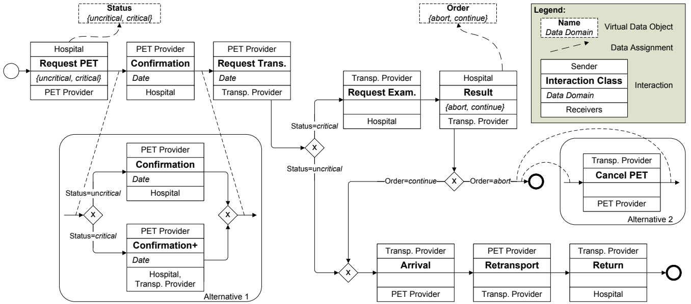
Fig. 2. Patient transportation scenario as DACHor
