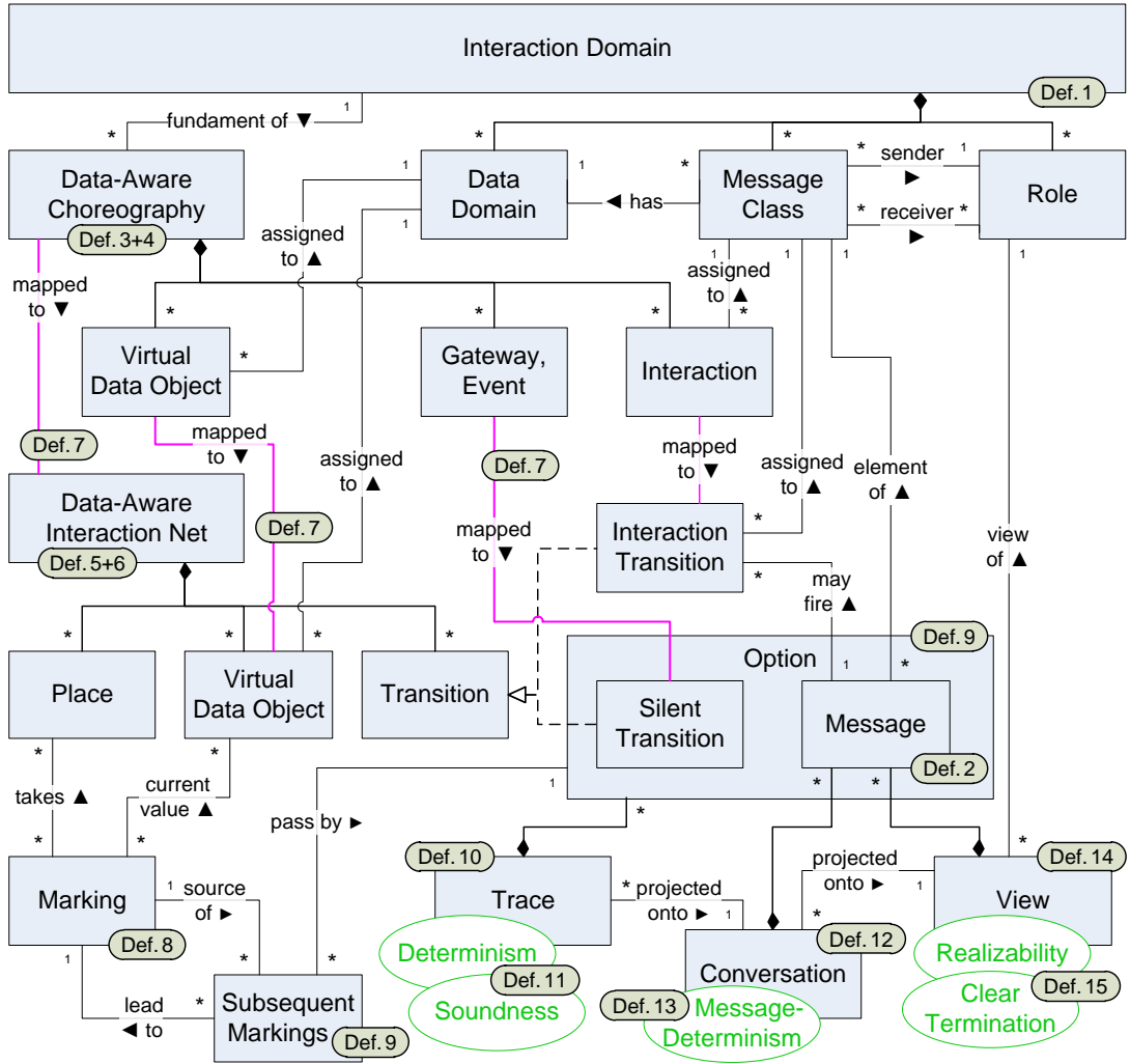
Fig. 3. Overview of our formal framework
