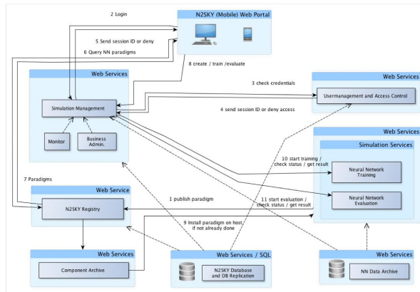
Figure 10: Previous N2Sky Architecture
