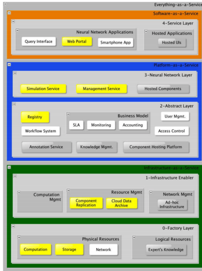
Figure 5: Previous N2Sky Architecture
